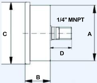
Panel / Back Mount Pressure Gauge
